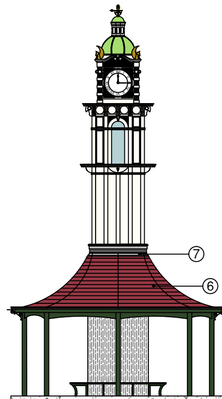
LEFT ELEVATION
