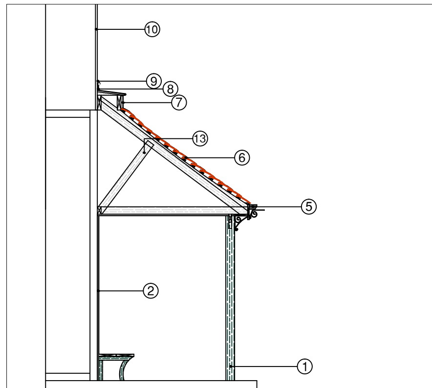
EXISTING SECTION THROUGH COLONNADE
